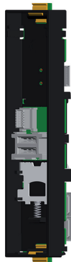
Supply module socket MS-S1-RD-TS 31.702.50
